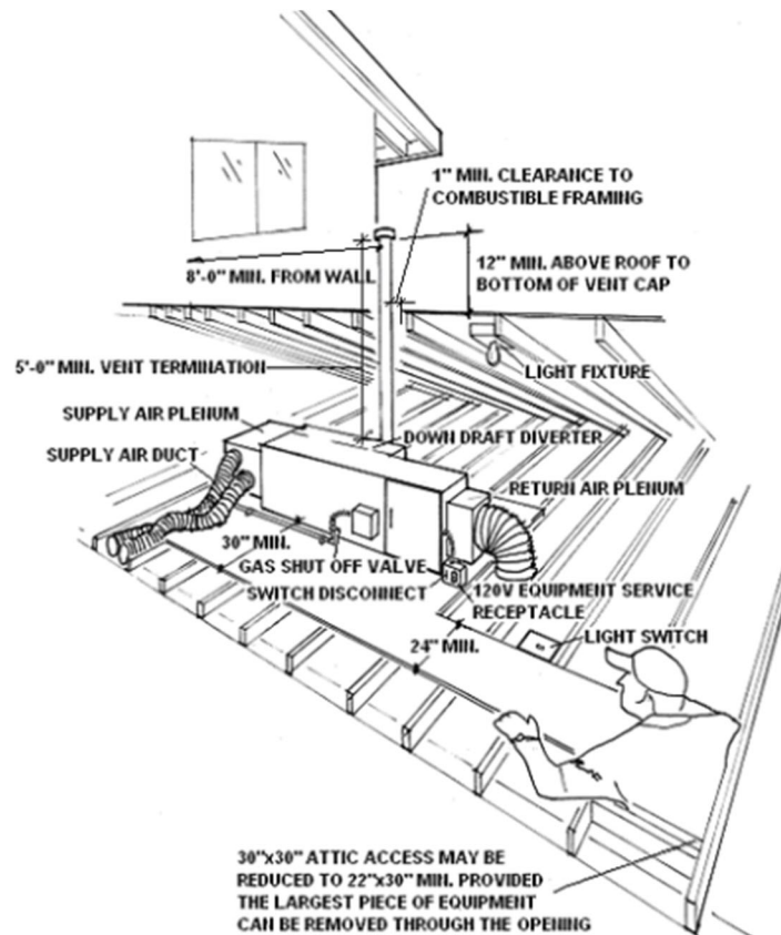
Figure 1 – Typical Installation of Forced Air Unit in Residential Project
