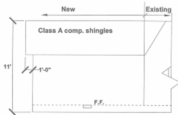
WEST Elev.
