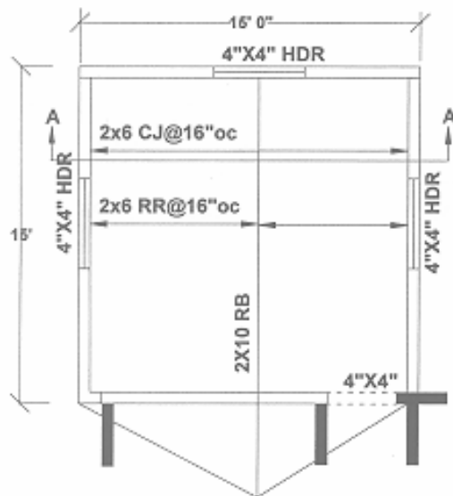
Roof Framing
